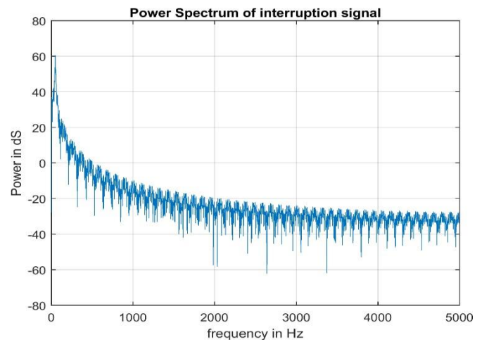
(b) Power Spectrum of interruption signal
