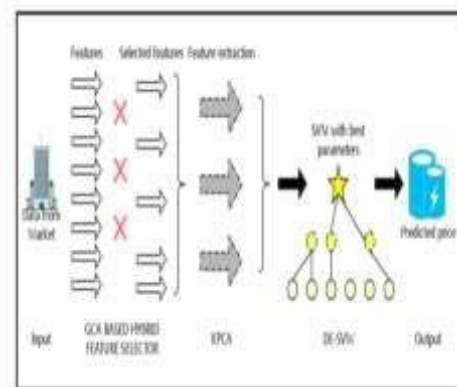
Fig. 1: Our proposed approach
