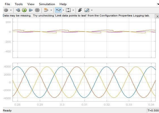
Fig.17: Electric vehicle current
