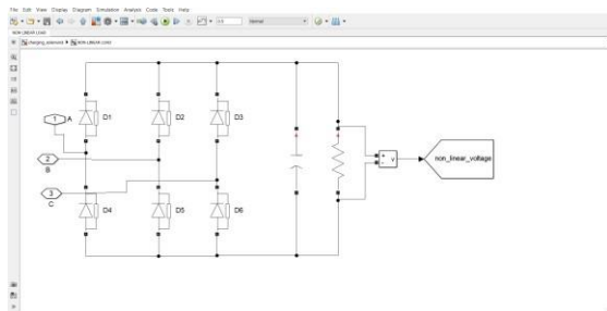
Fig.12: Nonlinear load
