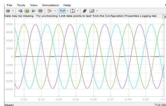
Fig.16: Load voltage
