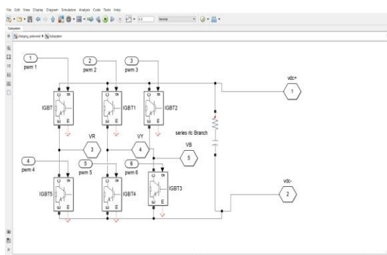
Fig.13: Inverter design
