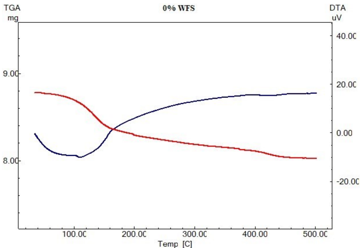
Figure 14. TGA and DSE curve graph for 0%WFS+ 100%MS
