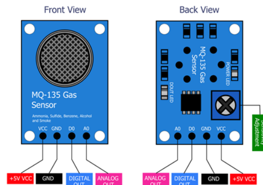
Figure 3: MQ135 Gas Sensor
