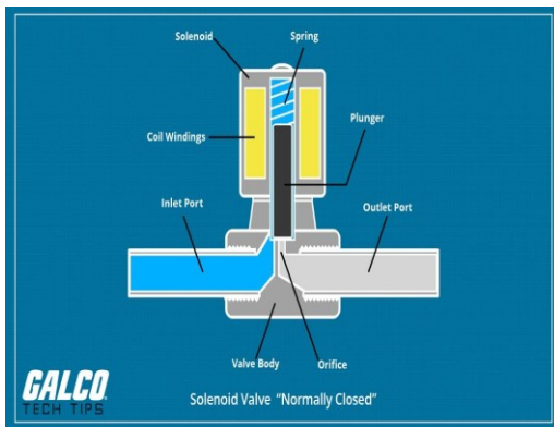
Figure 7: Solenoid Valve
