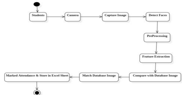
Fig2: Activity Diagram
