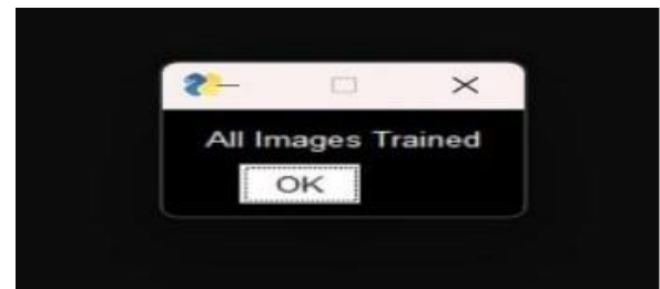
Fig8: Images Trained
