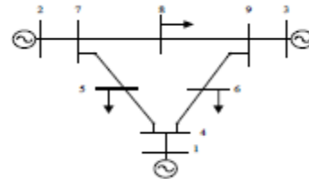
Figure 3. Structure of IEEE 9-bus system
