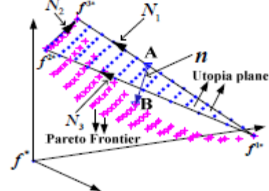
Figure 1. Utopia plane and Pareto optimal frontier for a three-objective case
