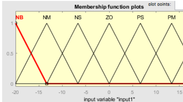
Fig.4. Speed error
