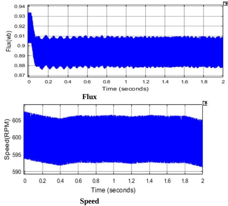
Fig. 10. Performance of IM with load torque equal to 0 (N.m) Rotor speed and stator flux amplitude under the proposed FLC based controller method
