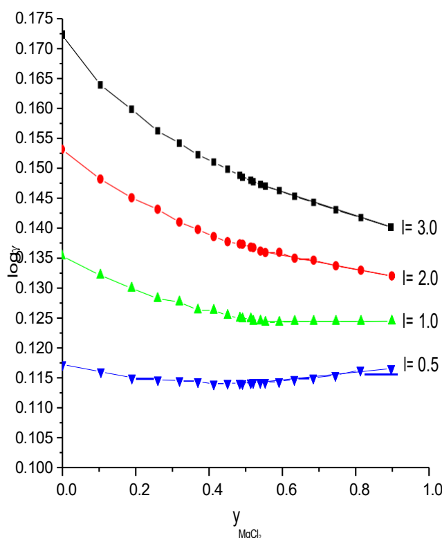
Graph1: Variation of -\log \gamma_{NaCl} with y_{MgCl_2} at 25^\circ C in the system NaCl-MgCl_2 -glycine- H_2O .
