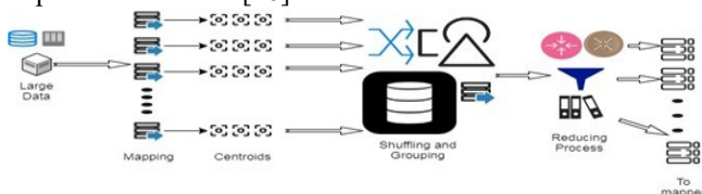
Fig.3.Map-Reducing Process [16]
