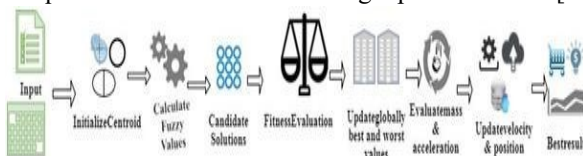
Fig.1.Fuzzy C-Means Technique [16]
