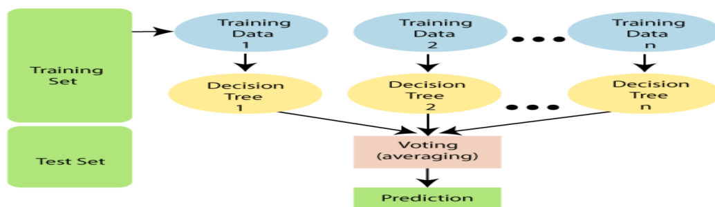
Fig.3. RFA network
