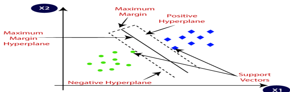
Fig.2. SVM network
