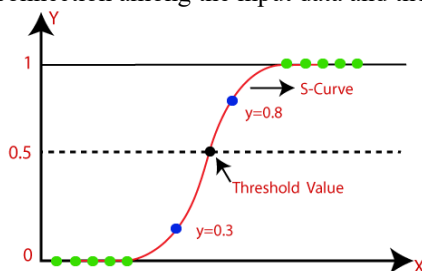
Fig.5. LR network
