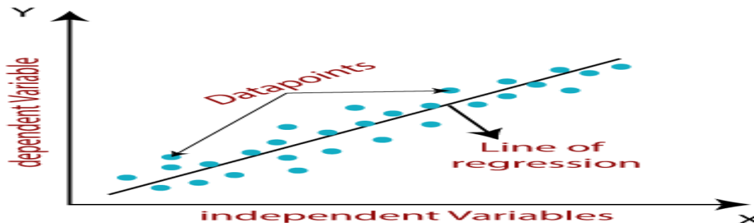
Fig.4. Regression's Network
