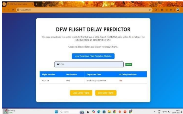
Fig4: delay predictor
