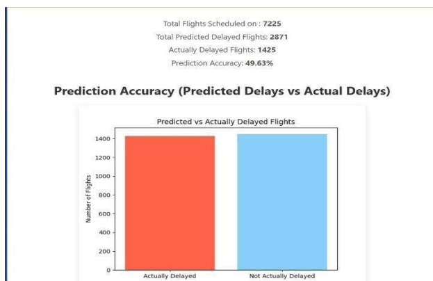
Fig5: predict
