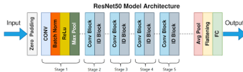
Figure 1: ResNet50 architecture
