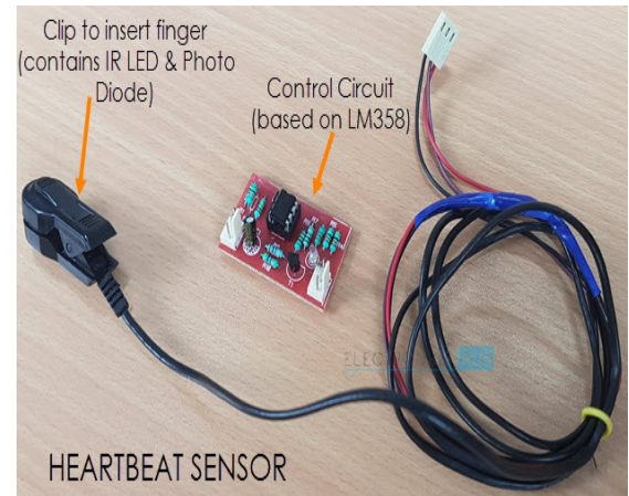
Fig Heart beat sensor
