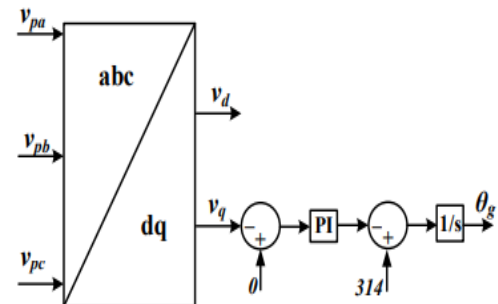
Fig. 4 Grid voltage phase angle estimation
