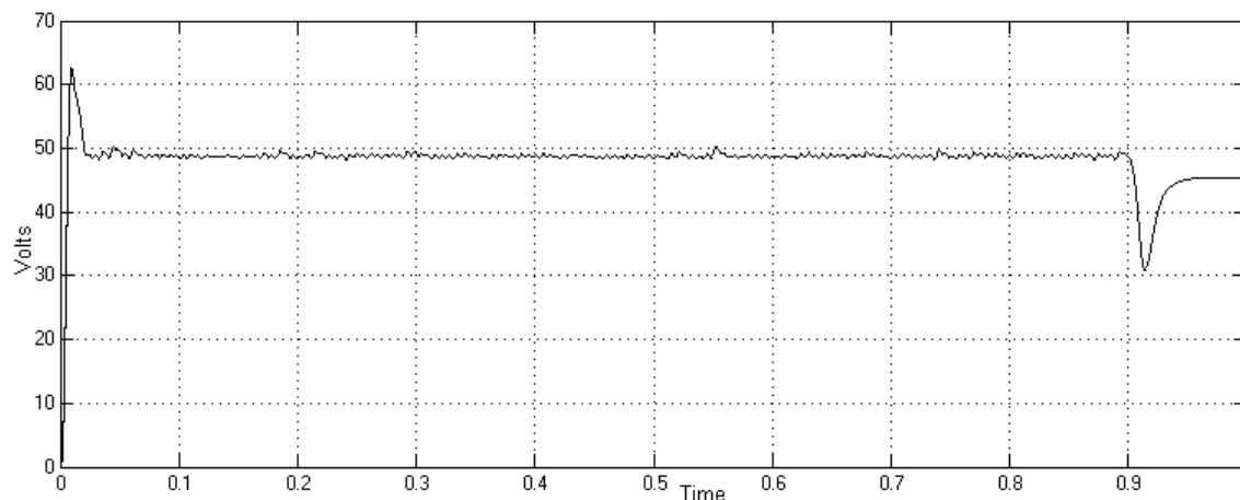
Fig. 11 Capacitor Voltage
