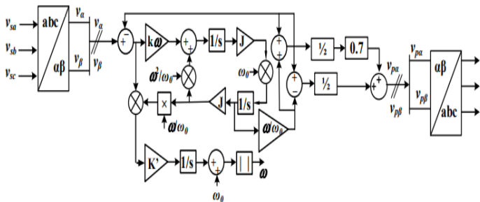
Fig. 3 estimating grid voltages in the positive sequence
