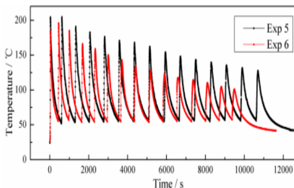
Figure 5. Comparison of thermal cycles of Point A in Exp 5 and Exp 6
