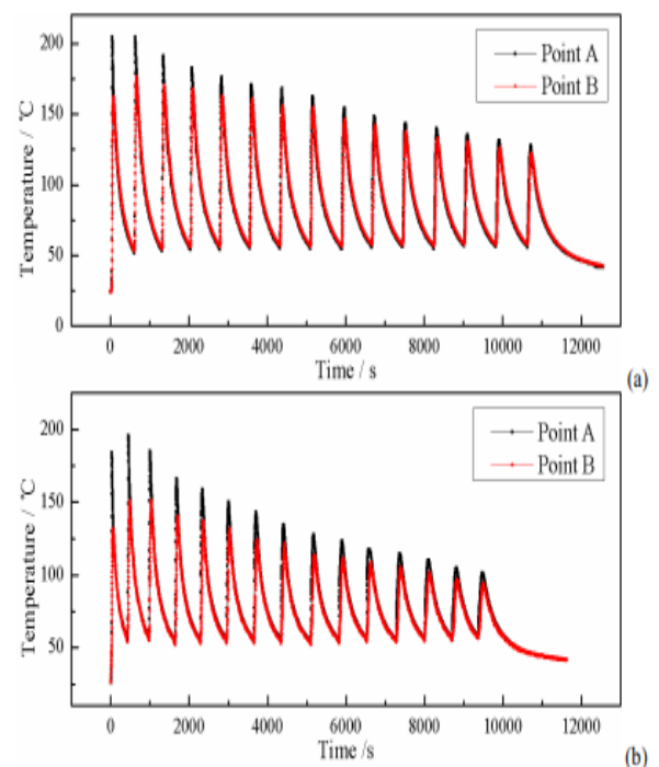
Figure 4. Thermal cycles of Point A and B in Experiment 5-6. (a) Exp 5. (b) Exp 6
