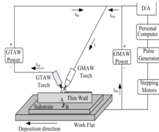
Figure 1. Schematic diagram of DE-GMAW based AM system.
